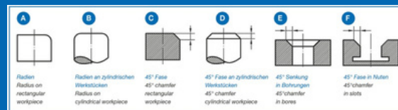
DIATEST KT / KT-B Chamfer Gauge
